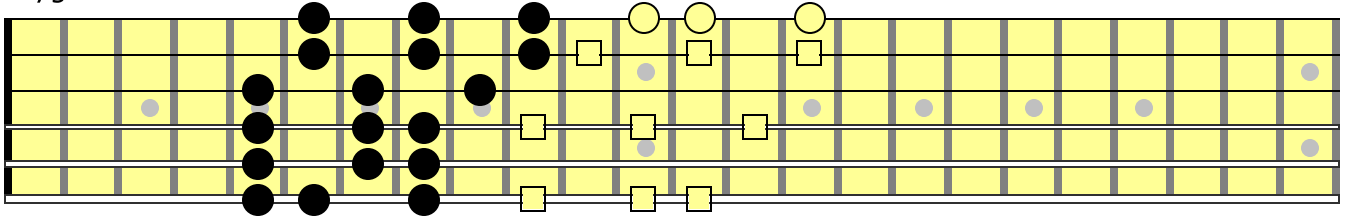
Frygian
